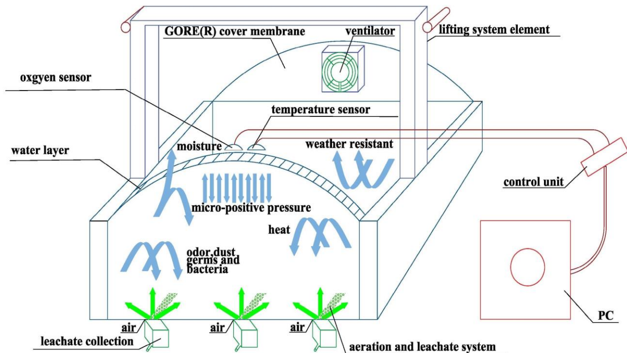
Figure 1. Schematic diagram of the encapsulated lifting system with GORE® Cover membrane
